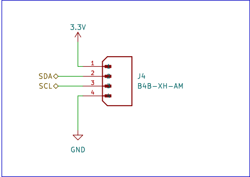
OLED display connector (I2C)
