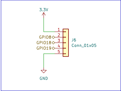
Breakout for remaining pins
