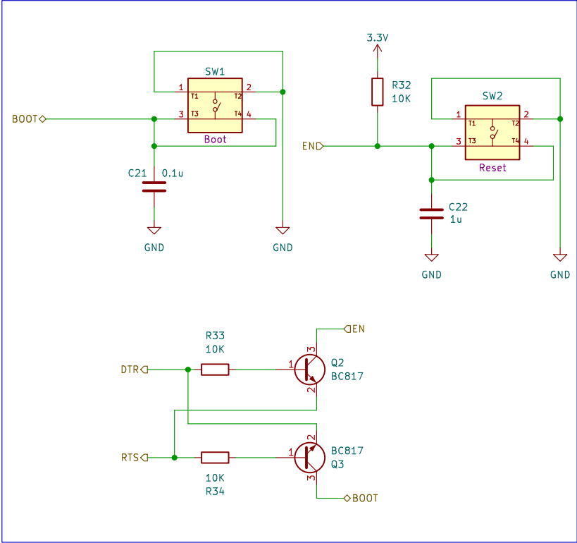
RESET and BOOT buttons
